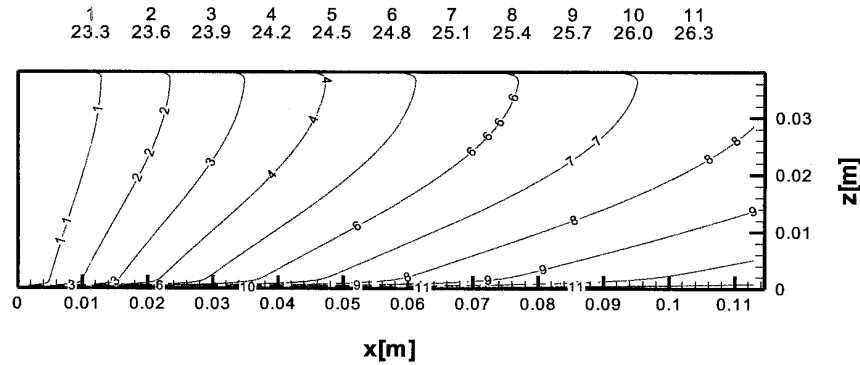
Sl. 3. Temperaturno polje v zraku pri Re_h = 1904 , T_m = 22,85\text{ }^\circ\text{C} , T_g = 26,64\text{ }^\circ\text{C} Fig. 3. Temperature fields in the air at Re_h = 1904 , T_m = 22,85\text{ }^\circ\text{C} , T_g = 26,64\text{ }^\circ\text{C}
