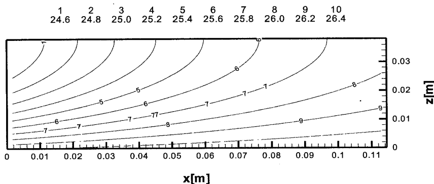
Sl. 2. Temperaturno polje v trdnini pri Re_h = 1904 , T_{in} = 22,85 °C, T_g = 26,64 °C Fig. 2. Temperature fields in the solid at Re_h = 1904 , T_{in} = 22.85 °C, T_g = 26.64 °C
